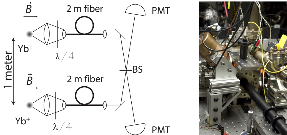
Figure 7: Bell inequality with two remote atomic qubits. The left-hand side is a schematic description of the experiment reported in [Matsukevich et al. (2008)Matsukevich, Maunz, Moehring, Olmschenk, and Monroe] in which the internal states of two ions separated by about one meter were entangled. Measurements on the two ions then allowed the violation of the CHSH inequality with the detection loophole closed. A series of laser pulses simultaneously excite both \text{Yb}^+ ions in such a way that when they deexcite, they emit a photon whose polarization is entangled with the ion. A lens is used to couple the photons into optical fibers. The wave plate ( \lambda/4 ) is used for convenience to convert circular polarization into linear polarization. The two photons interfere on a Beam Splitter (BS) and are detected by Photo Multiplier Tubes (PMT). Simultaneous detection of a photon by the two PMT's signals that the photons were in a Bell state, thereby realizing entanglement swapping: the two ions are now entangled. The internal states of the ions are then measured, enabling a violation of the CHSH inequality. Note that there are many inefficiencies in this experiment: only a fraction of emitted photons are coupled into the optical fibers, and only a fraction of the photons reaching the PMT's are detected. But when two photons are detected, one knows with certainty that the two ions are entangled. The right hand side is a photograph of one of the ion traps. The other trap is similar, and located about one meter away on the same optical table. (Both figures courtesy of S. Monroe and D. Matsukevich; left-hand side panel copyright American Physical Society).
